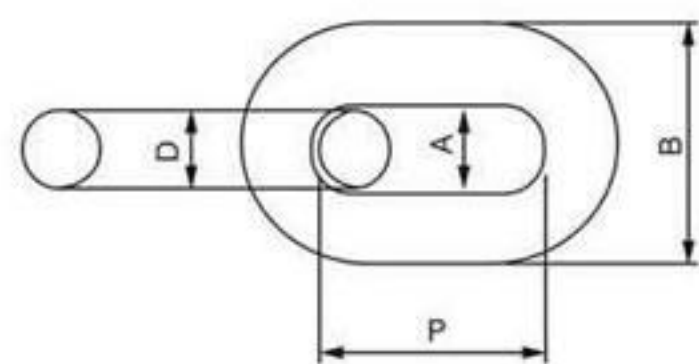
Chain 链条
